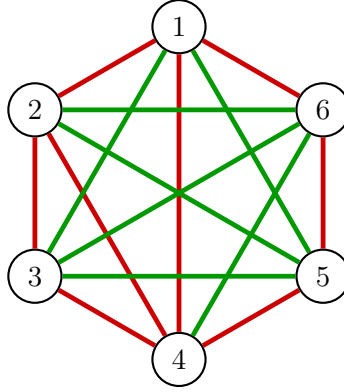
Figure 1: An example 2-colour colouring fulfilling Ramsey number R(3, 3) = 6 . Nodes 1, 3, 5 form a clique size 3. LaTeX code generated by Anthropic's Claude Sonnet 4.6
