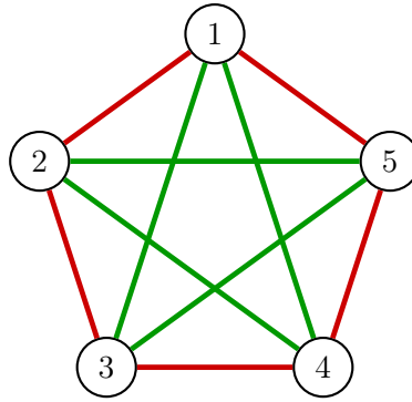
Figure 2: An example 2-colour colouring showing how 5 nodes is not enough. R(3, 3) > 5 . There is no monochromatic clique. LaTeX code generated by Anthropic's Claude Sonnet 4.6
